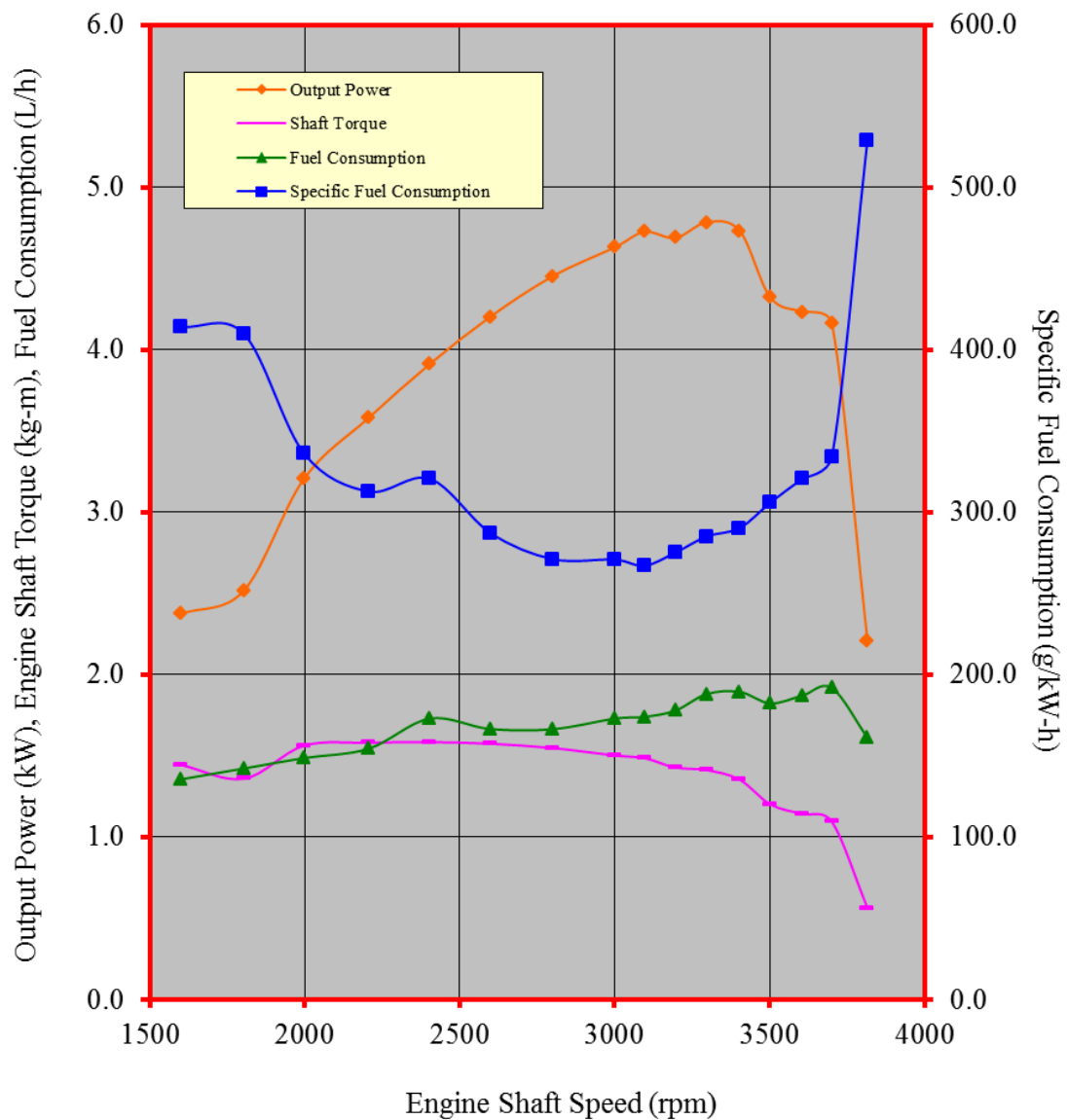
Figure 3. Performance characteristic curves of the LONCIN D350FD diesel engine
