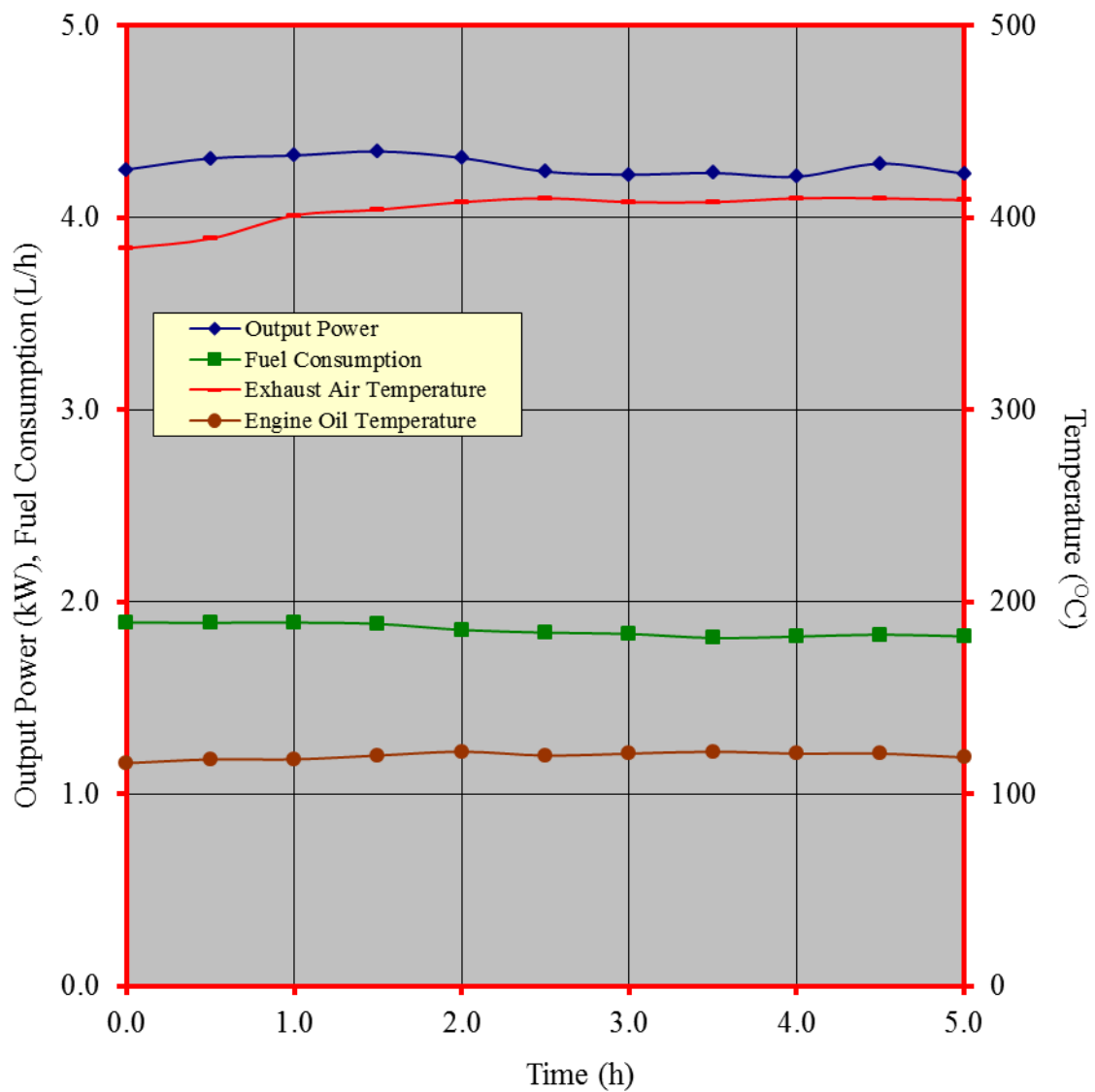
Figure 4. Performance characteristic curves during the continuous running test of the LONCIN D350FD diesel engine
